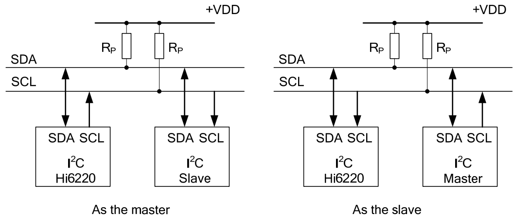
Figure 5-1 Typical I 2 C application circuit
